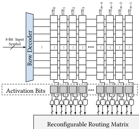
Figure 2. AP architecture. STEs are stored in a memory array, and edges are encoded in a reconfigurable routing matrix.
